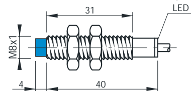
Kurzbauforn / Short Housing
